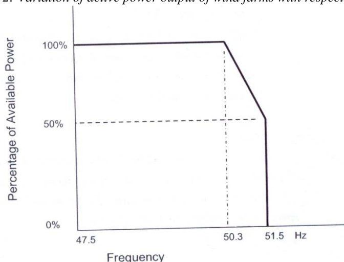
Figure 2: Variation of active power output of wind farms with respect to frequency
