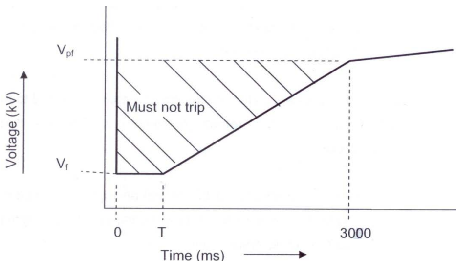
Figure 3: Fault ride through characteristics
