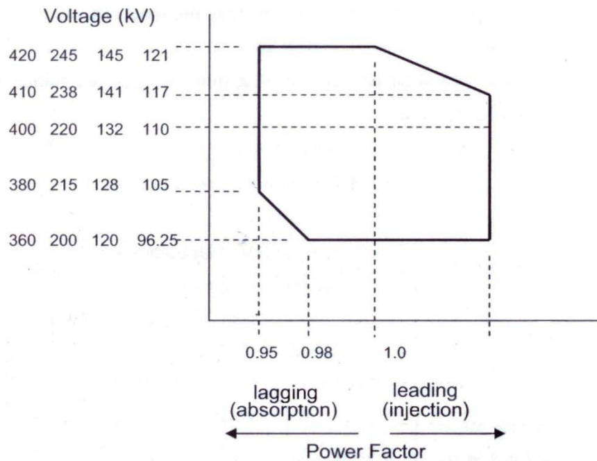
Figure 1: Voltage vs. power factor characteristics of wind farms connected above 66 kV
